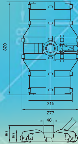
BE18 Bendervac
